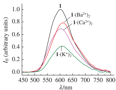
Figure 2 Quantum-corrected fluorescence spectra of dye 1 and the 1 ·(Ba 2+ ) 2 , 1 ·(Ca 2+ ) 2 , and 1 ·(K + ) 2 complexes in MeCN at 293 K. The relative areas in the fluorescence spectra correspond to the ratios of the underlying \varphi_f values.
