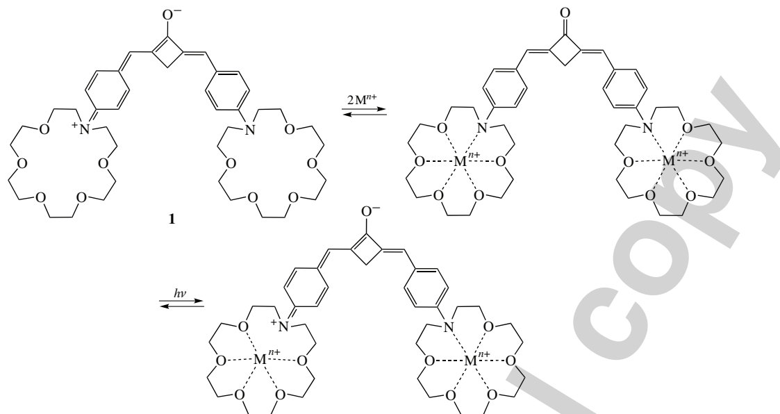
Scheme 1 Quinonoid form of dye 1 , complex 1 -(M n+ ) 2 , (M n+ = Ba 2+ , Ca 2+ , K + ) in the ground and excited states (after recoordination).
