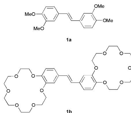
Scheme 1 Structure of donors 1a and 1b .
