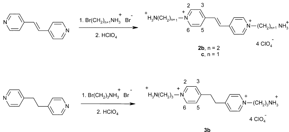
Scheme 2 Synthesis of acceptors 2b , c and 3b .
